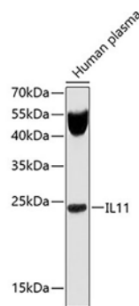
Fig. 1. Western blot analysis of extracts of Human plasma, using IL11 antibody at 1:1000 dilution. Secondary antibody: HRP-labeled Goat Anti-Rabbit IgG(H+L) (A0208) at 1:1000 dilution. Lysates/proteins: 25µg per lane. Blocking buffer: QuickBlock™ Blocking Buffer (P0231). Detection: BeyoECL Star (P0018A). Exposure time:1s.
